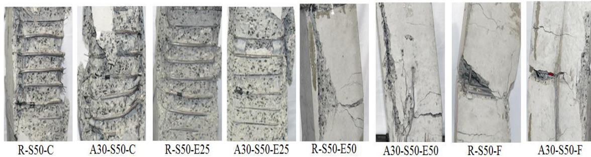
Figure 2 Failure modes of the tested specimens
