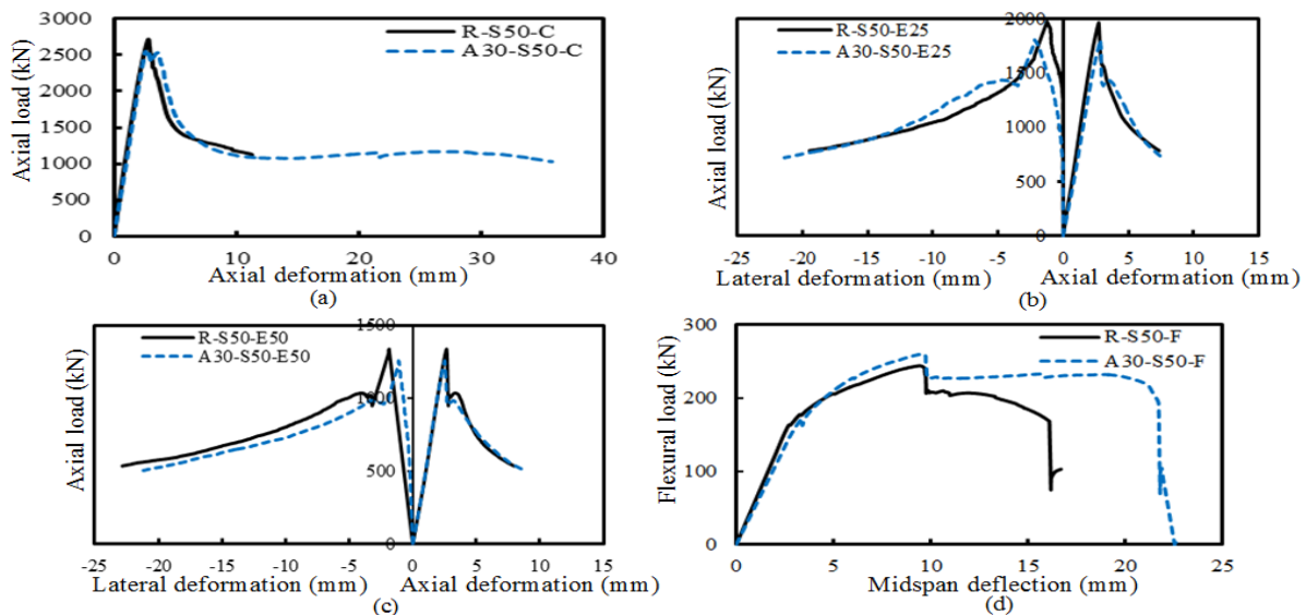
Figure 3 Test results of specimens under (a) concentric axial load (b) 25 mm eccentric axial load (c) 50 mm eccentric axial load and (d) four-point bending
