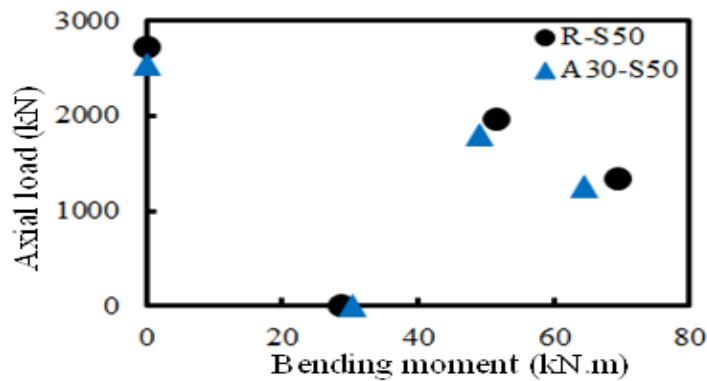
Figure 3 Experimental axial load-bending moment interaction diagram of specimens
